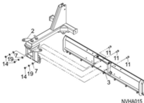
Figure 12. Turn Table Installes to Moldboard.
