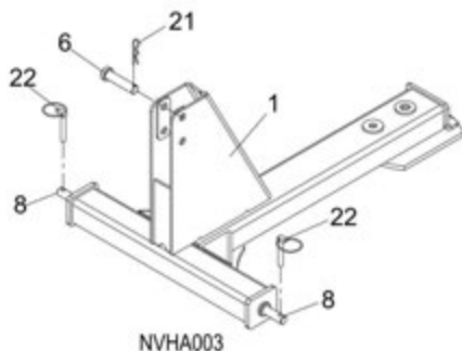
Figure 1. 3-point Hitch Connection
