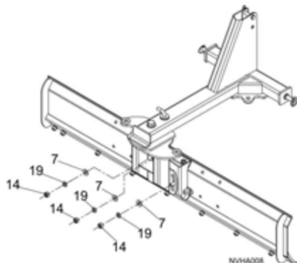
Figure 6. Upper Turn Table Pin
