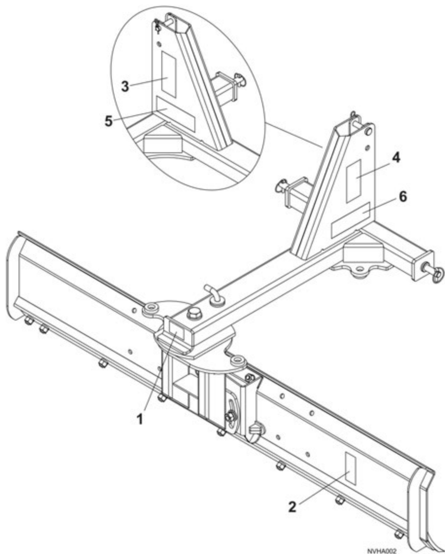
1 - Serial Number Plate (1)
