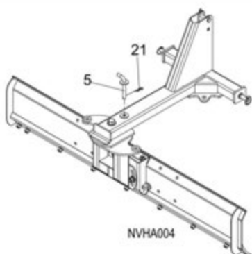
Figure 2. Turn Table Pin
