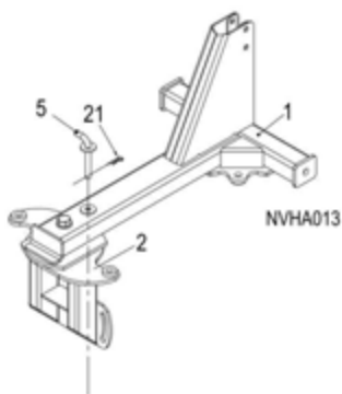
Figure 10. Upper Turn Table Pin Installation
