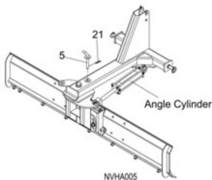
Figure 3. Hydraulic Angle Cylinder
