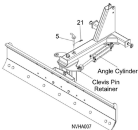
Figure 5. Adjustment Hydraulic Angle Cylinder
