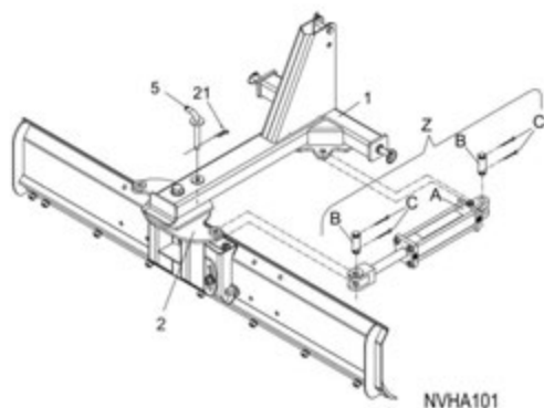
Figure 14. Angle Cylinder Installation
