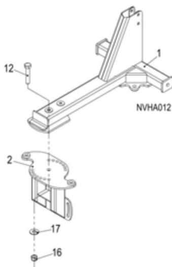
Figure 9. Turn Table Installed to Main Frame
