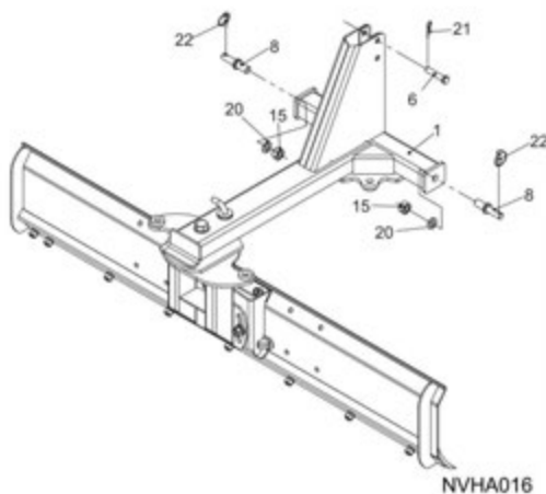
Figure 13. 3-Point Hitch Mast and Main Frame Pin Installation
